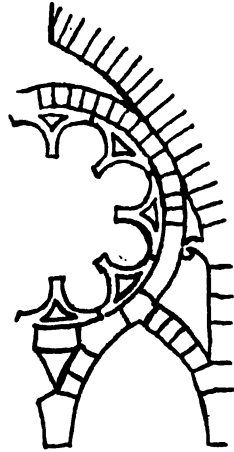
FIG. 79. Construction of early traceried windows, c. 1220, Amiens Cathedral.
